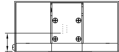
LOWEST ORIFICE .81 ON 1/2" PRINT HEAD .61 ON 7/8" PRINT HEAD
